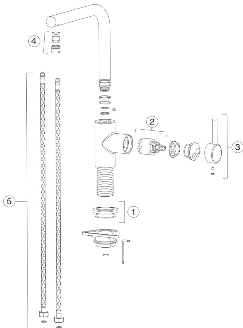
Tap Lina L Swivel side HP CO
