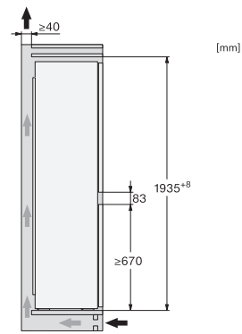
KFN7913E, side view
