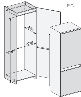
KFN7913E, built-in
