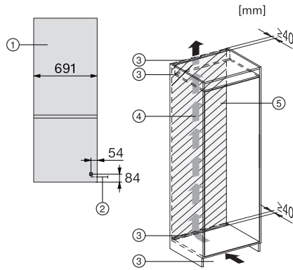
KFN7913E, installation
