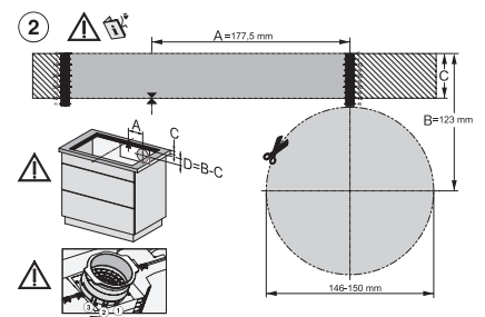
KMDA7272-1FL/FR, KMDA7473-1FL/FR, KMDA7272FL/FR, KMDA7473FL/FR – Installation variant 11 Exhaust air
