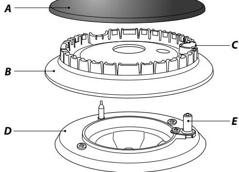
A – Kap, B – Kop, C – Inkeping, D – Basis, E – Elektrode
